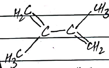
2,3-Dimethyl-1,3-butadiene \lambda_{\text{max}} = 225\text{nm}
